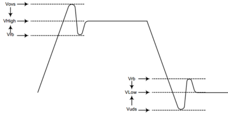
Figure 1.1. PCIe Single-Ended Signal Integrity Limits
