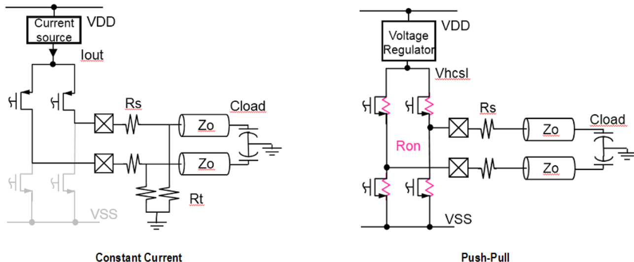
Figure 2.1. PCIe Clock Driver Types
